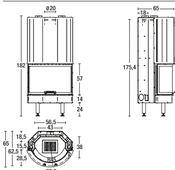
Model: 760T
