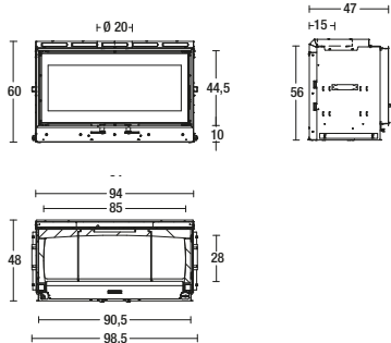
Model: MC 90/44
