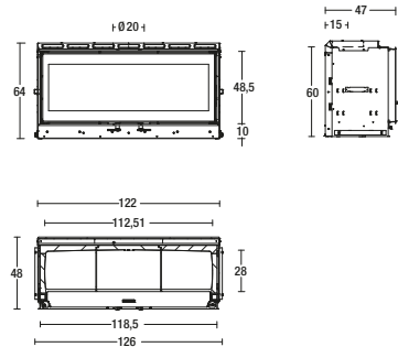
Model: MC 120/48
