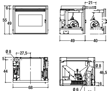
Model: IP 7
