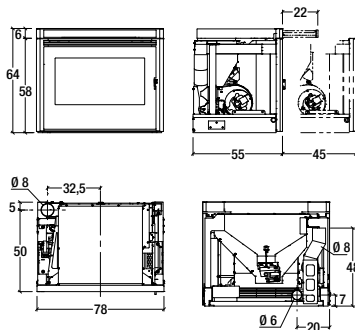
Model: IP 9
